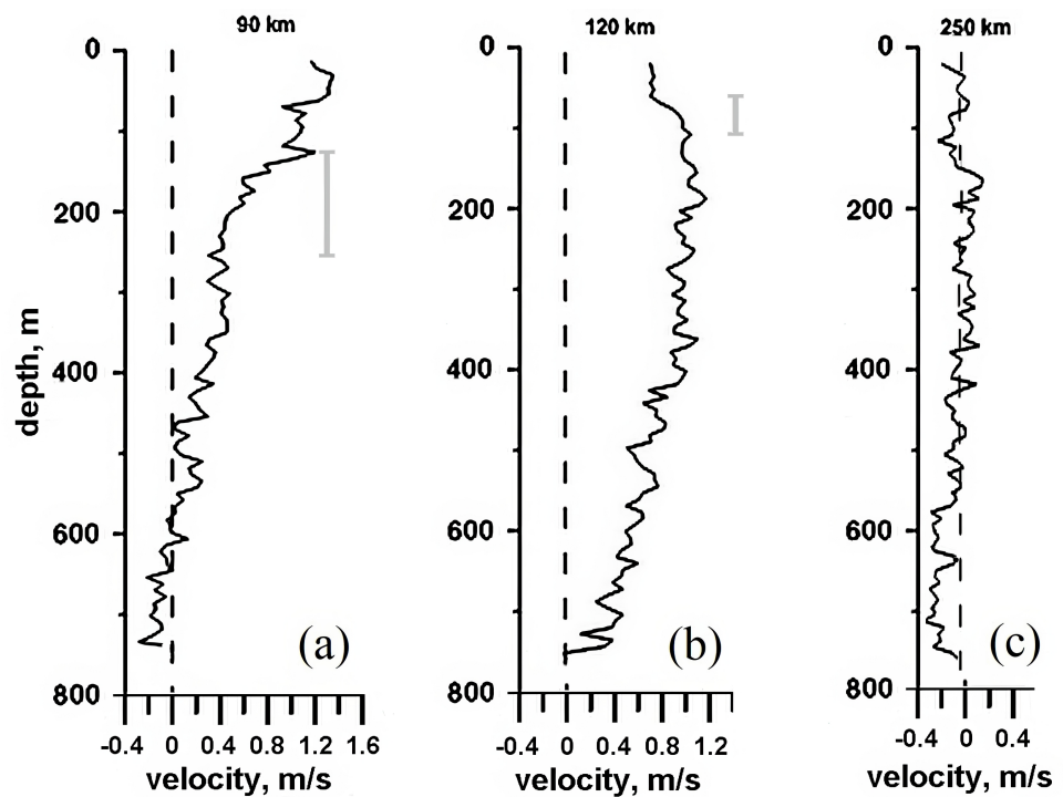
Figure 11. Vertical profiles of longitudinal velocity at three points of the section in 2015. Locations of profiles are shown in Figure 9: (a) 39.87°N; (b) 39.66°N; (c) 38.65°N. Gray bars mark the intervals for assessing vertical gradients.
