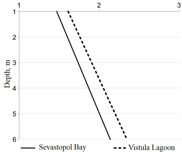
Figure 8. Dependencies of methane solubility on the depth of the station for the Sevastopol Bay ( S = 18\text{‰} ) and the Vistula Lagoon (average depth 2.7 m, S = 3.8\text{‰} ) at a water temperature of 22 °C.
