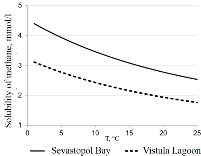
Figure 7. The calculated dependence of the solubility of methane in pore waters on the water temperature for the Sevastopol Bay (average depth 11.3 m, S = 18\text{‰} ) and the Vistula Lagoon (average depth 2.7 m, S = 3.8\text{‰} ) calculated by Henry's Law.
