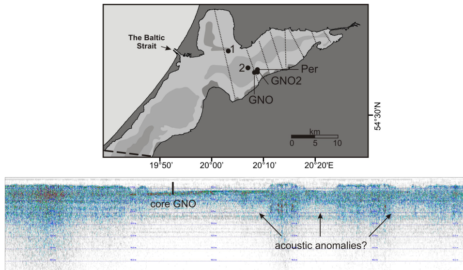
Figure 3. Map of the coverage of the Vistula Lagoon with geoaoustic profiles with a two-channel Knudsen Chirp 3212 profilograph (3.5–210 kHz) and the location of sampling stations (above); geoaoustic signs (acoustic transparency) of gas saturation of bottom sediments of the Vistula Lagoon, obtained on a profile through the GNO station.
