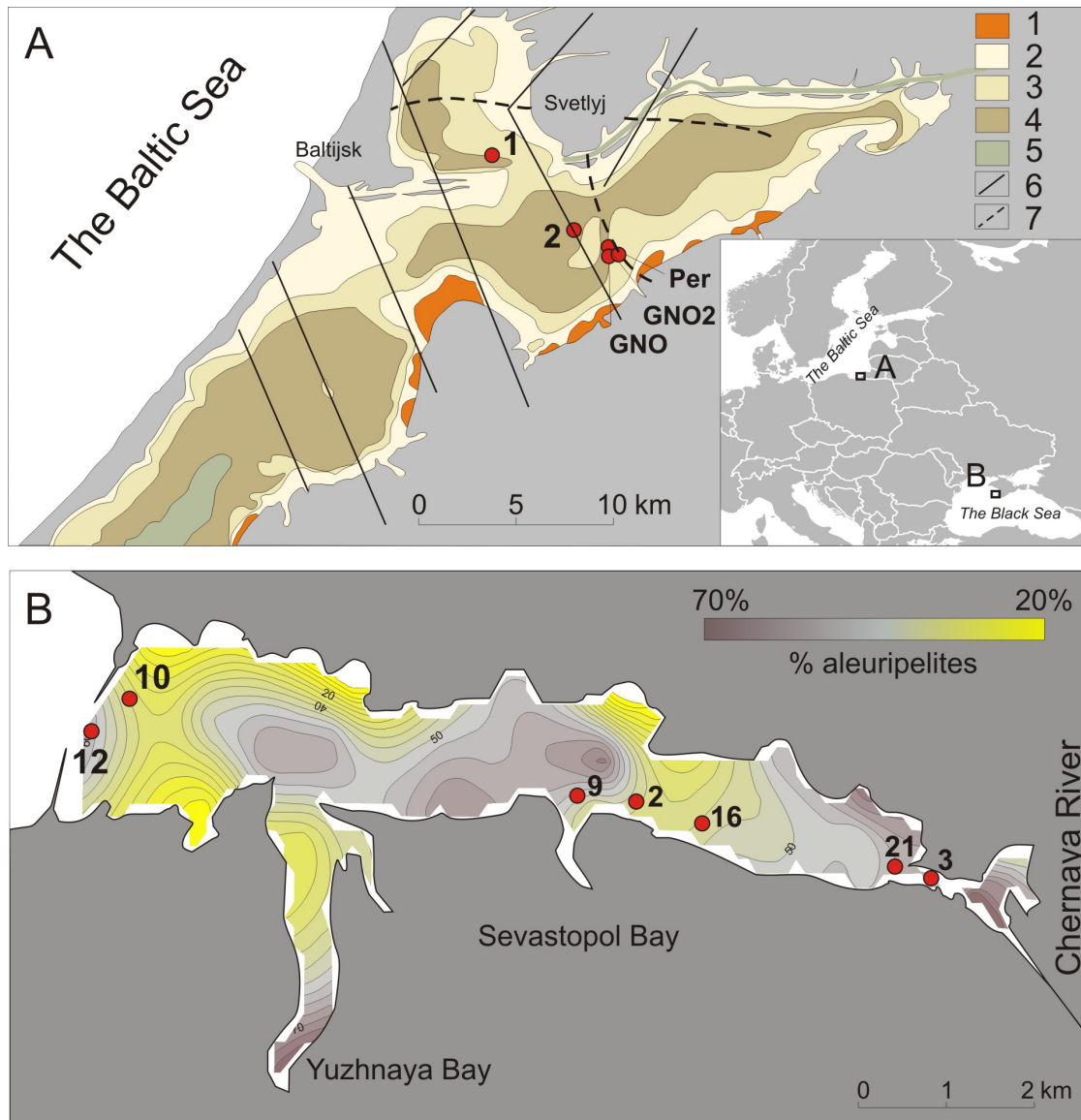
Figure 1. Map of the study areas in the Black and Baltic Seas; A) Station location and types of bottom sediments in the northeastern part of the Vistula Lagoon (Baltic Sea), surface layer 0–7 cm [Chechko, 2006]; B) The distribution of the finely dispersed fraction (% aleurite-pelite), surface layer 0–5 cm [Moiseenko et al., 2010] and the location of the stations in the Sevastopol Bay (Black Sea); Legend: 1 – boulder-gravel; 2 – sand; 3 – large aleurite; 4 – fine silt; 5 – aleurite-pelitic mud; 6 – faults [Dunaev, 2018]; 7 – borders of tectonic elements of the second order [Otmaz et al., 2017]
