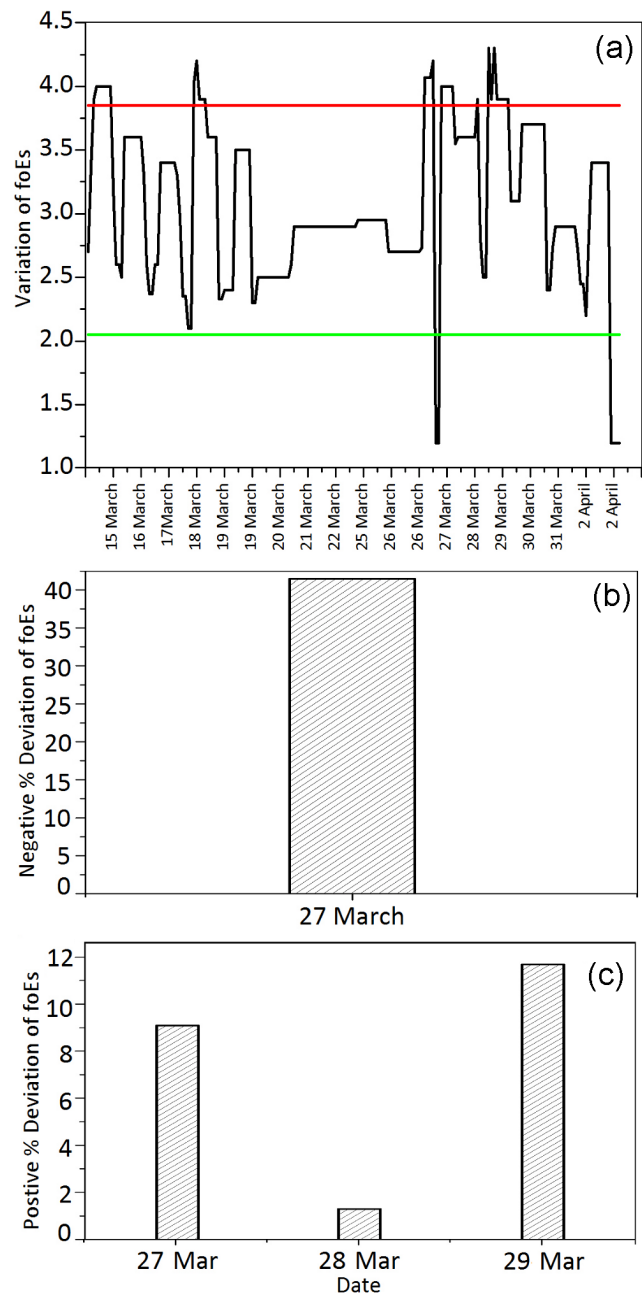
Figure 3. a – Variation of f_oE_s parameter for Jicamarca Station from 15 March to 2 April 2014; b – Percentage deviation of f_oE_s parameter of Jicamarca Station on 27 March 2014; c – Percentage deviation of f_oE_s parameter of Jicamarca Station on 27th, 28th and 29th March 2014.
