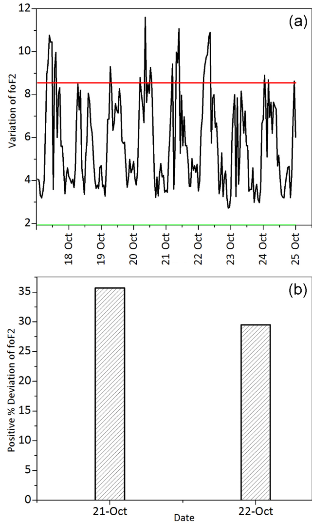
Figure 5. a – Variation of f_oF2 parameter of Kokubunji Station from 17 October to 25 October 2013; b – Percentage deviation of f_oF2 parameter of Kokubunji Station on 21 October and 22 October 2013.
