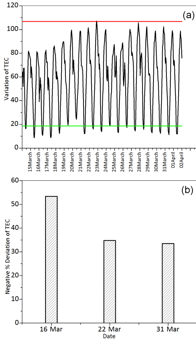
Figure 2. a – Variation of TEC parameter of Iquique Chile Station from 15 March 2014 to 2 April 2014; b – Percentage deviation of TEC for Iquique Chile Station on 16th, 22nd and 31st March 2014.
