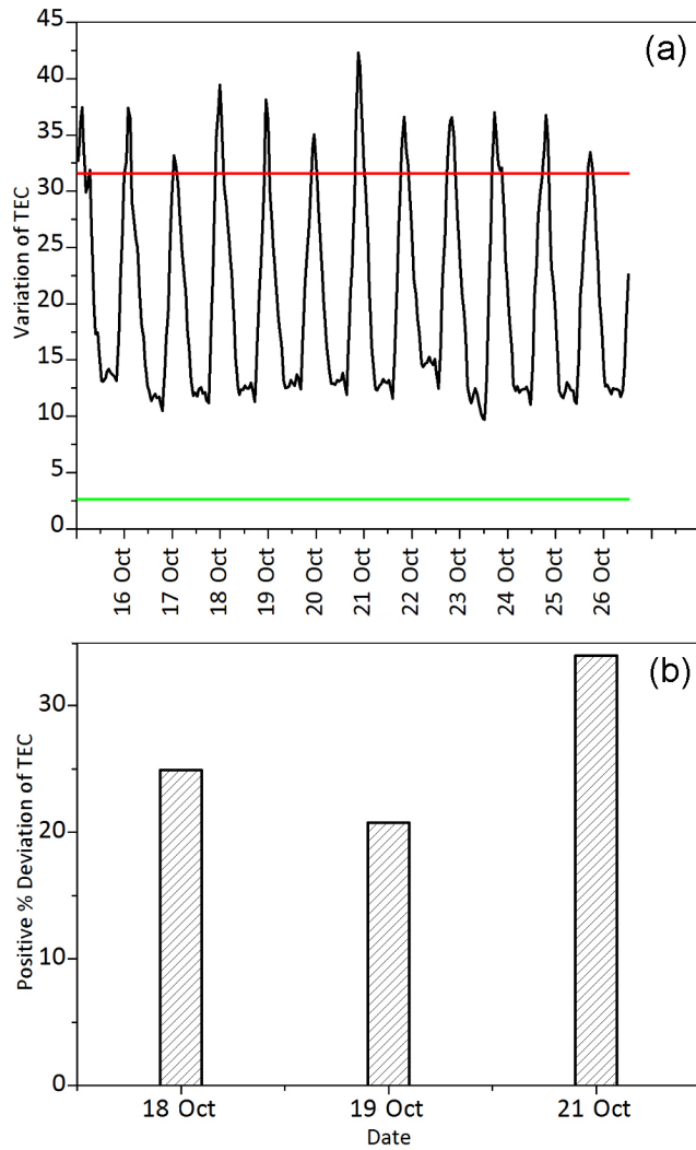
Figure 6. a – Variation of TEC parameter of Kashima Station from 15 October to 26 October 2013; b – Percentage deviation of TEC of Kashima Station on 18th, 19th and 21st October 2013.
