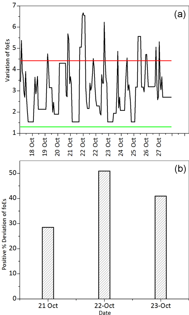
Figure 7. a – Variation of f_oE_s parameter of Kokubunji Station from 18 October to 27 October 2013; b – Percentage deviation of f_oE_s parameter of Kokubunji Station on 21st, 22nd and 23rd October.
