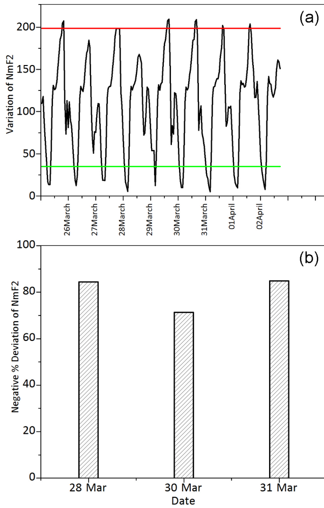
Figure 4. a – Variation of peak electron density ( N_mF2 ) parameter of Jicamarca Station from 25 March to 2 April 2014; b – Percentage deviation of N_mF2 parameter for Jicamarca Station on 28th, 30th and 31st March 2014.
