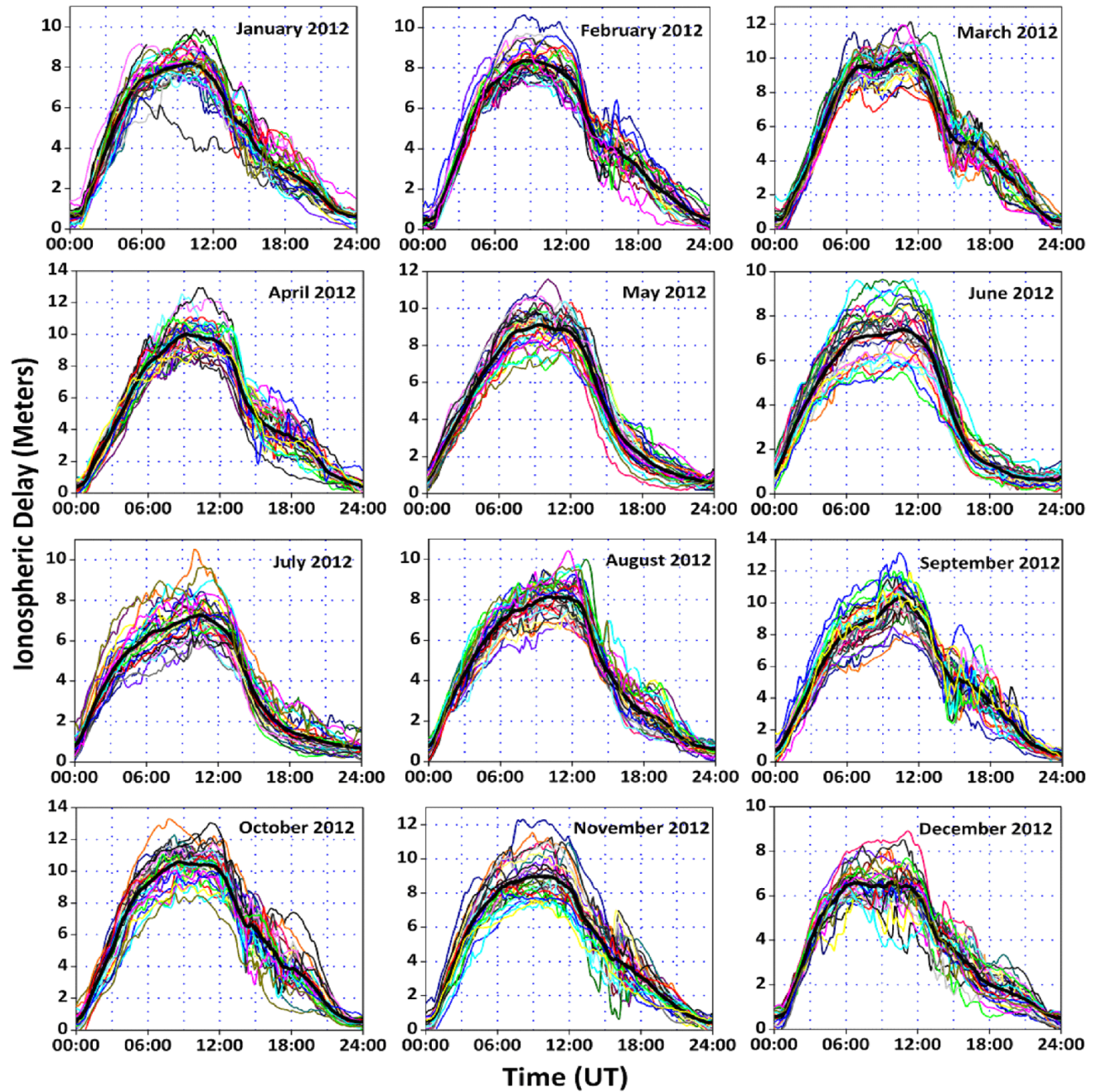
Figure 2. The diurnal variability of the ionospheric delay during all the months of the year 2012.
