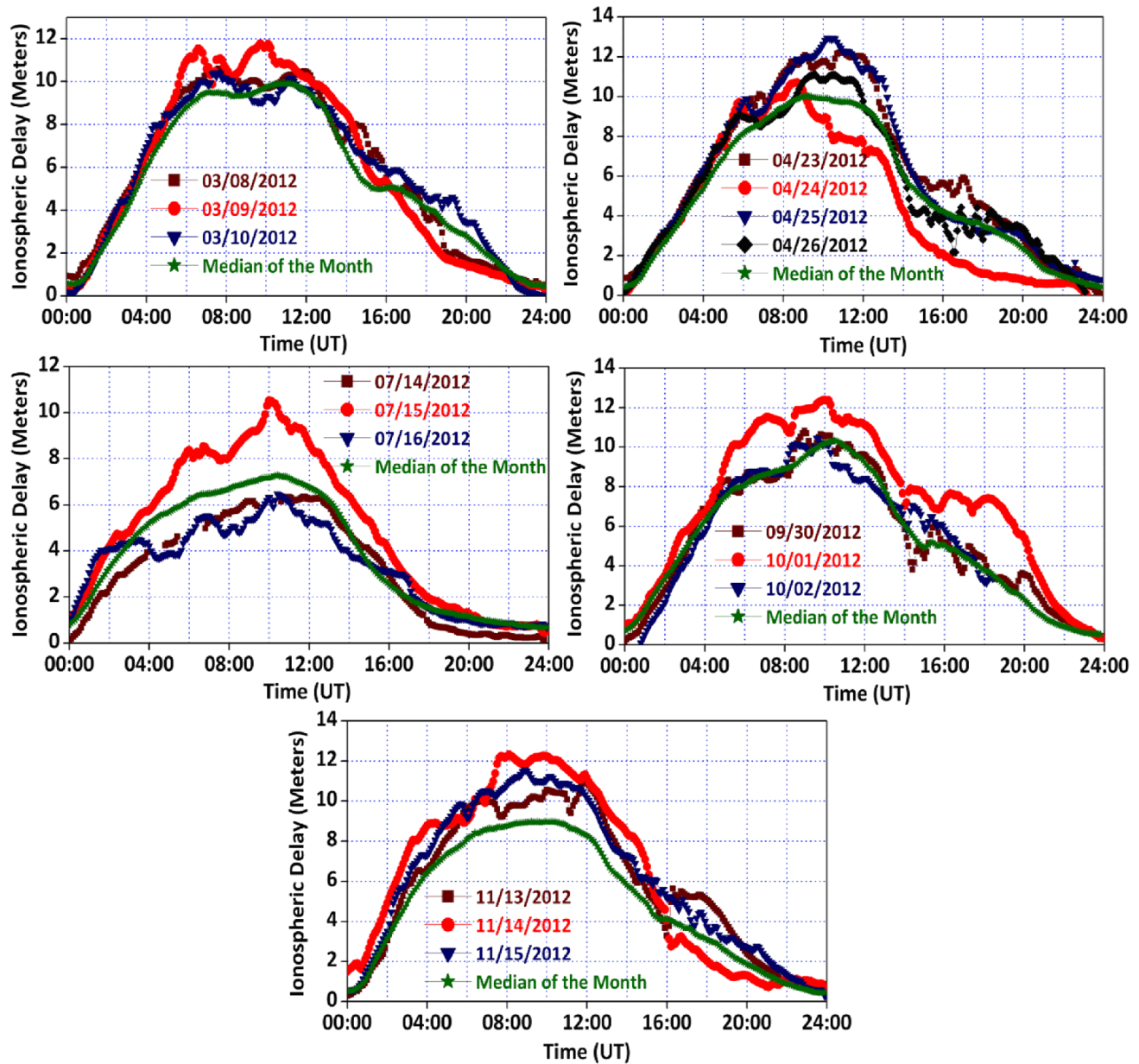
Figure 9. Diurnal time profile of ionospheric delay on the storm day, control day and on the day of median of the month during all the five selected storm events.
