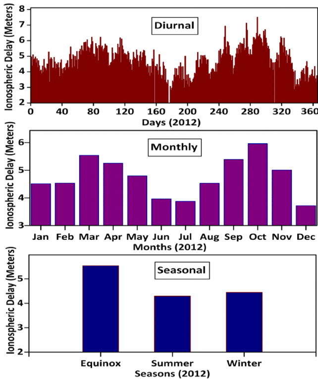
Figure 3. The diurnal, monthly and seasonal variability of the ionospheric delay during the year 2012.
