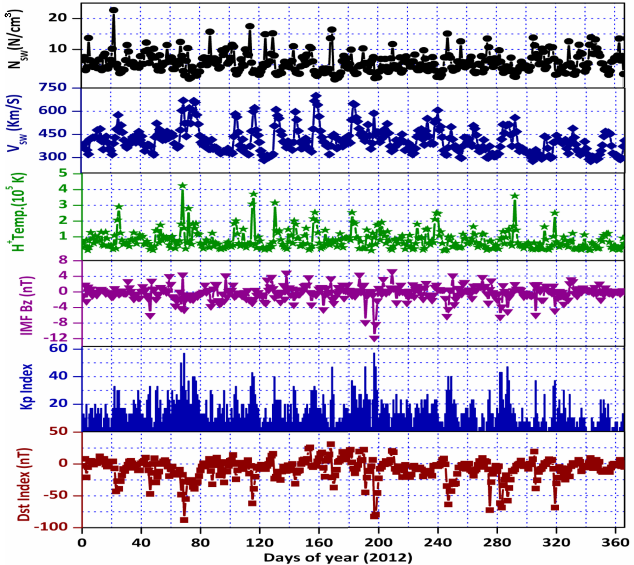
Figure 1. The daily behaviour of various geomagnetic and interplanetary indices during the year 2012.
