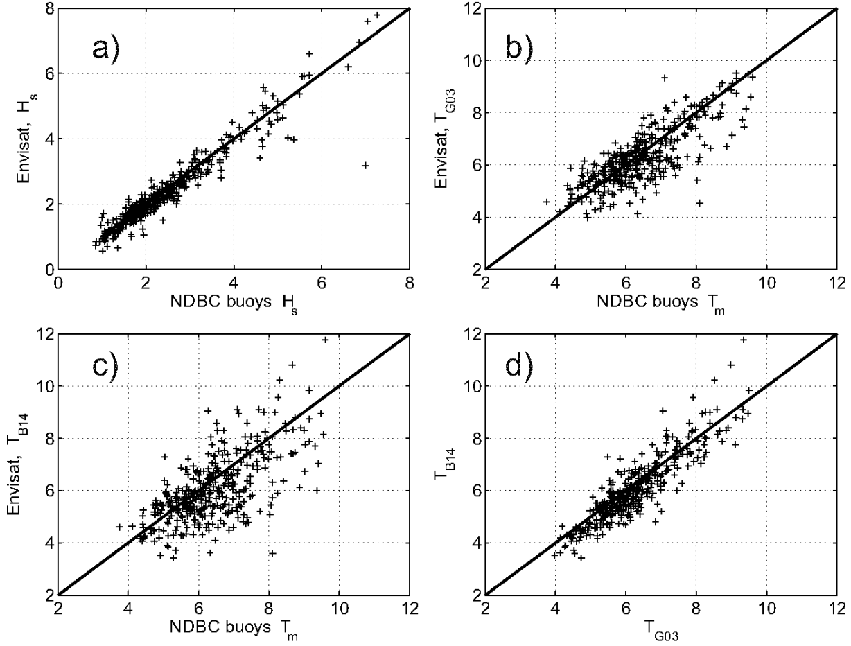
Figure 2. Scatter diagrams for altimeter (Envisat, 2011) and in situ NDBC buoys measurements for the Globwave database of match-ups. a) – significant wave heights (SWH); b) – mean-over-spectrum wave periods T_m measured by buoys (abscissa) and altimeter (ordinate) estimated by the parametric model G03; c) – mean-over-spectrum wave periods T_m measured by buoys (abscissa) and altimeter (ordinate) estimated by the physical model B14; d) – wave periods of G03 vs those of B14 model.
