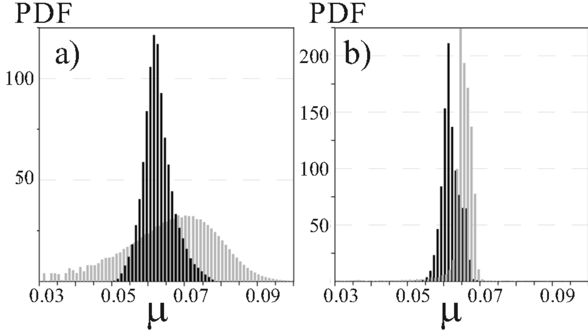
Figure 6. Probability density functions (PDF) for wave steepness estimates made within the parametric model G03 and the physical one by B14. a) – PDF for individual estimates of wave steepness; b) – PDF for the set of 2^\circ \times 2^\circ averaged wave steepness.
