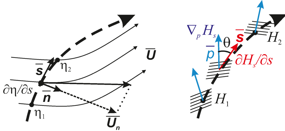
Figure 1. Left – setup of measurements of large-scale currents by satellite altimeter; right – setup of estimate of wave steepness from two consecutive along-track measurements of significant wave height by satellite altimeter. Different colors are used for along-track (red) and wave (blue) directions.
