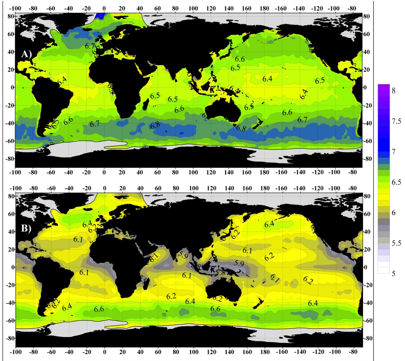
Figure 5. Global distribution of wave steepness derived from Envisat data in 2011. Top – physical model B14; bottom – parametric approach G03. Wave steepness values are multiplied by 100.
