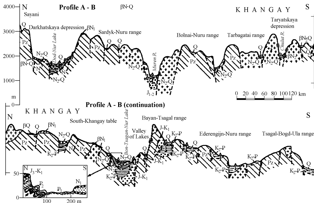
Figure 11. Geologic/geomorphologic profile through Mongolia, constructed by E. V. Devyatkin. After [Grachev, 2000].
