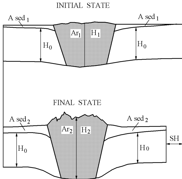
Figure 2. Previous scheme of crustal shortening determination from crustal thickening, after [Avouac et al. , 1993].
