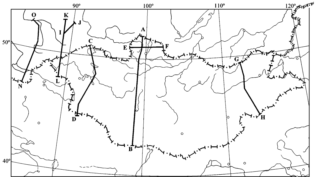
Figure 10. Location of profiles in Altay and Mongolia.
