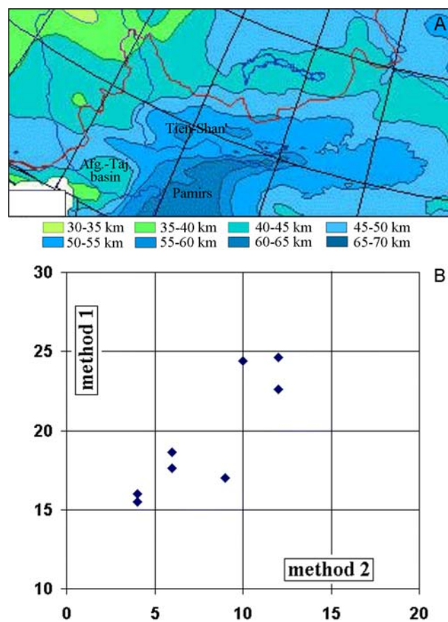
Figure 8. A – depths to Moho in the Pamir–Tien Shan region, after [Grachev, 2000], and B – comparison of shortening evaluations (percent) from Methods 1 and 2.
