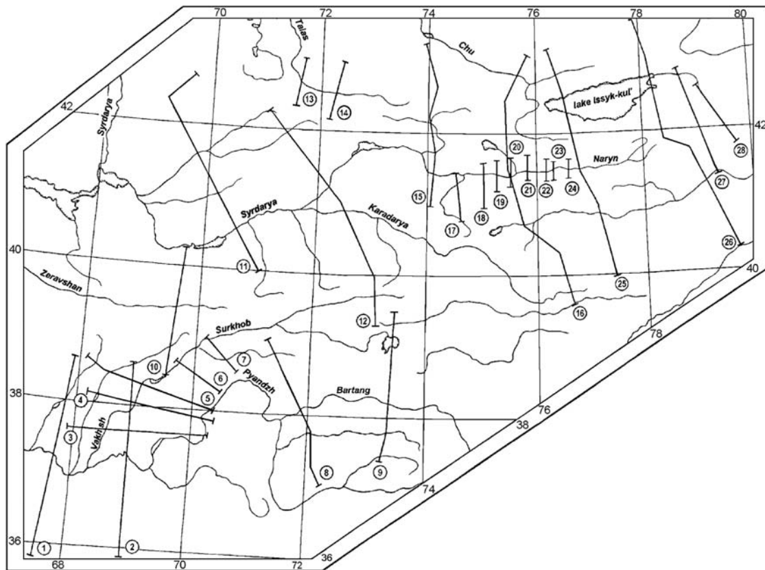
Figure 6. Location of measurement profiles across the Tien Shan, Afghan-Tajik basin, and Pamir structures.
