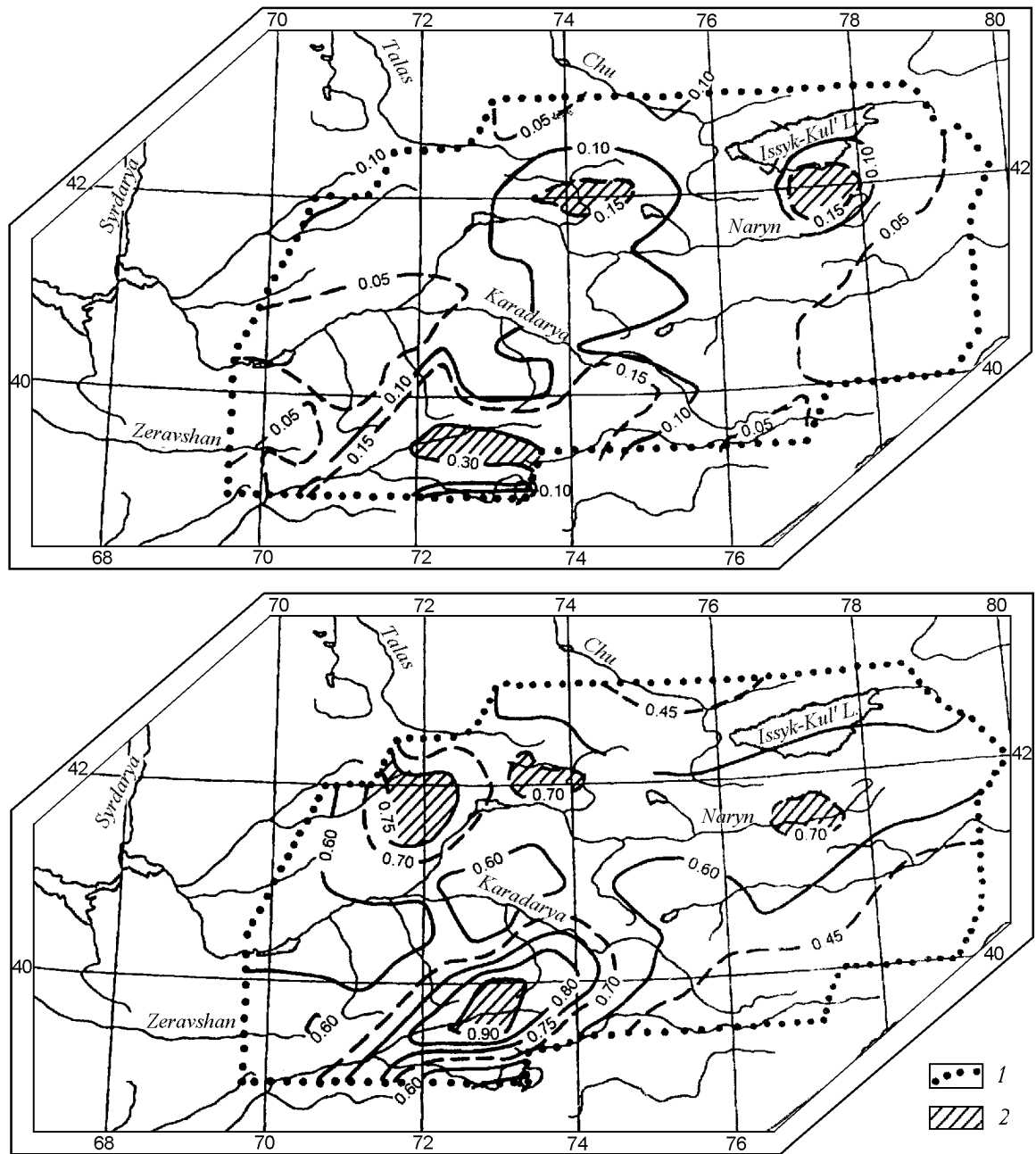
Figure 7. Areal distribution of crustal shortening values for Tien Shan, normalized from 0 to 1 for each data set [Grachev, 2000]. Top, shortening from penneplanation surfaces (F. L. Yakovlev) and bottom, shortening from crustal thickening (S. L. Yunga). 1 – boundary of data sets under comparison, 2 – local deformation maxima.
