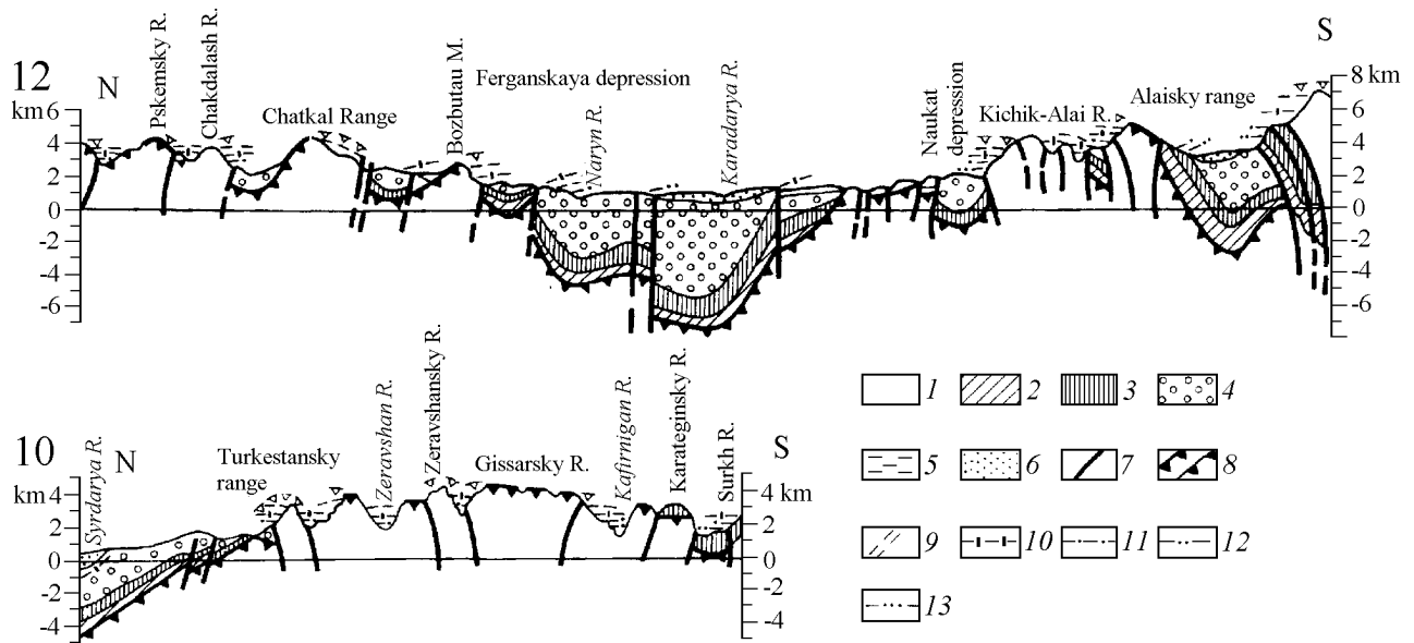
Figure 5. Structural profiles constructed by Chediya [1986]. Fivefold vertical exaggeration. 1 – pre-Mesozoic deposits undivided; 2 – Jurassic deposits; 3 – Cretaceous–Paleogene deposits; 4 – Cenozoic molasse; 5 – Middle Pleistocene deposits; 6 – Late Pleistocene to Holocene deposits; 7 – regional neotectonic faults; 8–13 – peneplained surfaces: 8 – pre-orogenic peneplain (initial peneplanation surface); syn-orogenic peneplanation surfaces (terraces, pediments) of different ages: 9 – Neogene, 10 – Early Pleistocene, 11 – Q_1 , 12 – Q_2 , and 13 – Q_3 .
