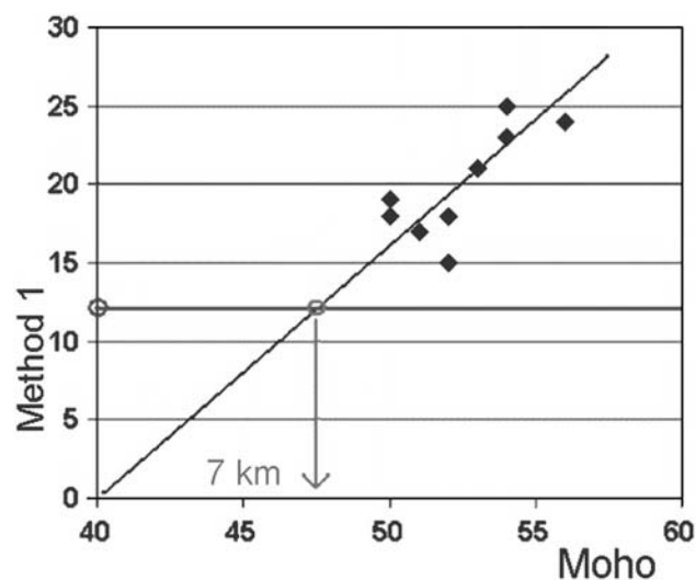
Figure 9. Comparison of shortening evaluations from N–S transects using Method 1 and averaged Moho depths from the same transects. Determination of crustal underplating.
