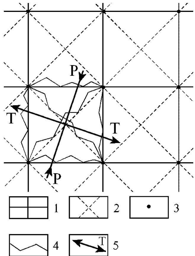
Figure 3. Schematic representation of calculations of shortening orientations and magnitudes from depths to Moho and neotectonic movement magnitudes. From S. L. Yunga’s data [Grachev, 2000].
