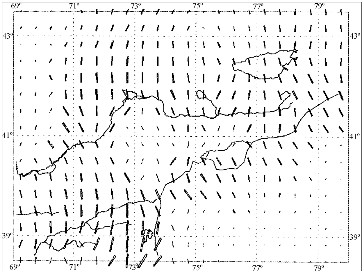
Figure 4. Orientations of main axes of compressional deformation, as determined from the Neotectonic Map of Northern Eurasia (From S. L. Yunga's data [Grachev, 2000]). Length of bars is proportionate to shortening amounts.
